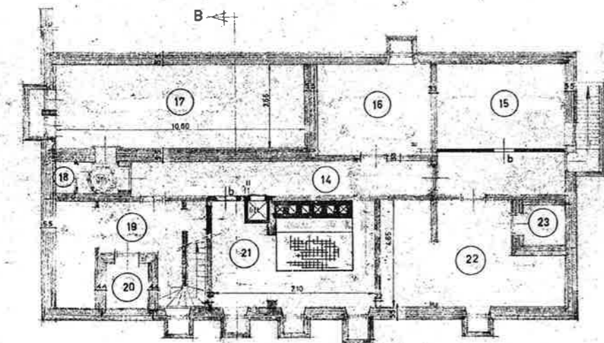
FIG.3. KELDER
