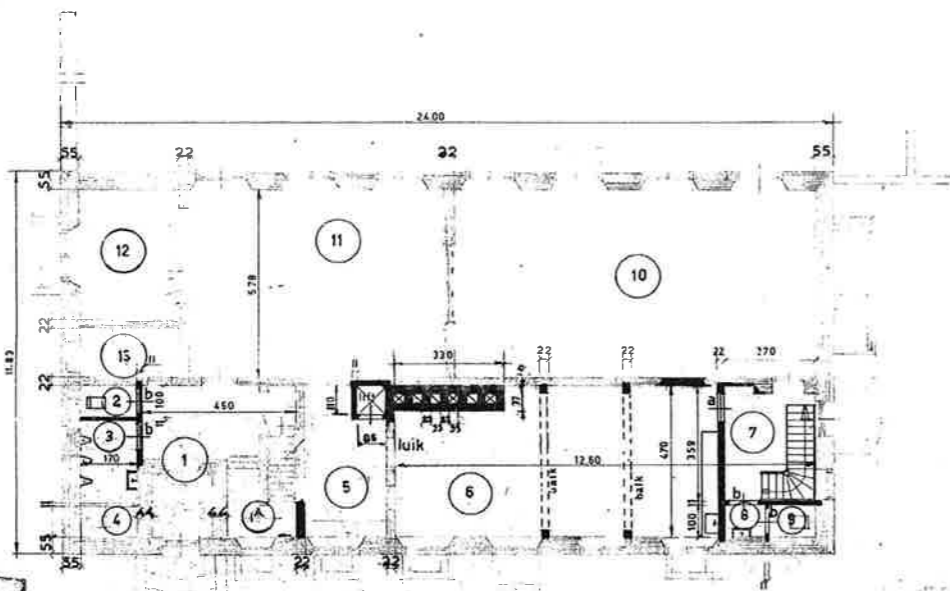
FIG.2. BEGANE - GROND
